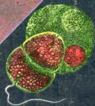
Glenodinium sanguineum , March.
